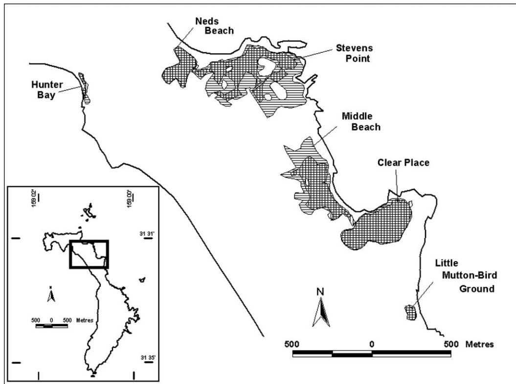
Fig. 1 – Location of the nesting grounds of the flesh-footed shearwater on Lord Howe Island in 1978 (horizontal hatching) and 2002 (vertical hatching).
