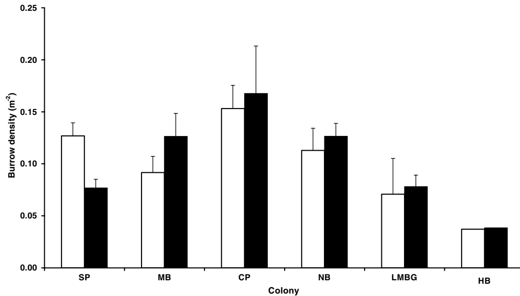
Fig. 2 – Burrow densities in flesh-footed shearwater colonies on Lord Howe Island in 1978 and 2002. SP, Stevens Point; MB, Middle Beach; CP, Clear Place; NB, Neds Beach; LMBG, Little Mutton-bird Ground; HB, Hunter Bay. 1978, unshaded columns; 2002, shaded columns.
